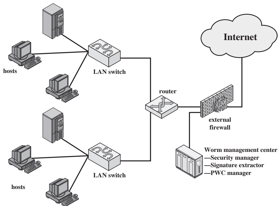
Figure 21.7 Example PWC Deployment
